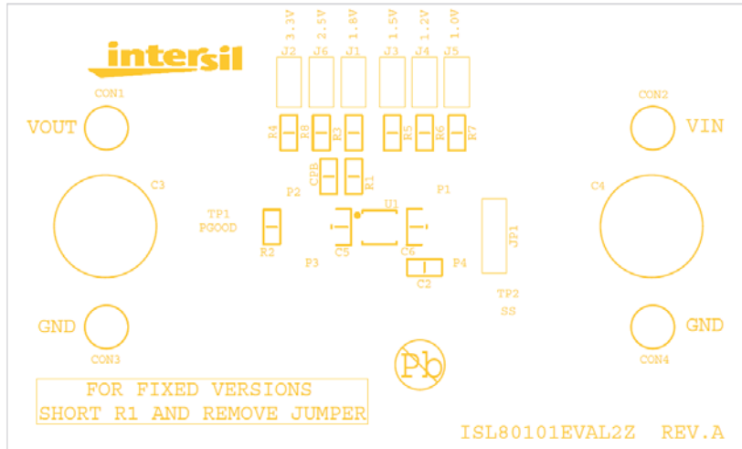
FIGURE 18. ISL80101EVAL2Z COMPONENT PLACEMENT
