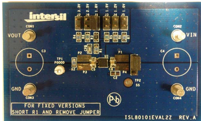
FIGURE 1. ISL80101EVAL2Z
